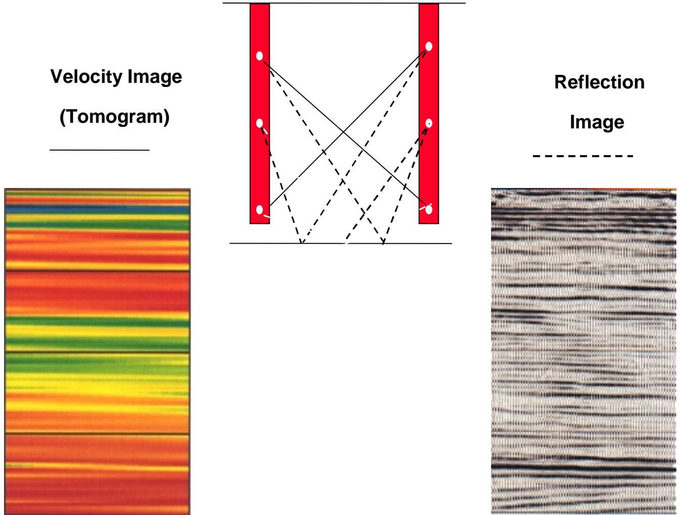
Figure 4. Typical raypaths for direct and reflected arrivals.
